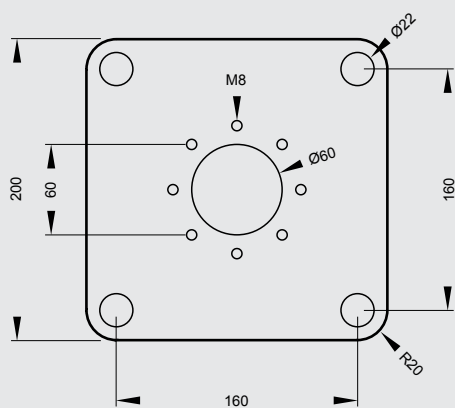
Adapterplate
