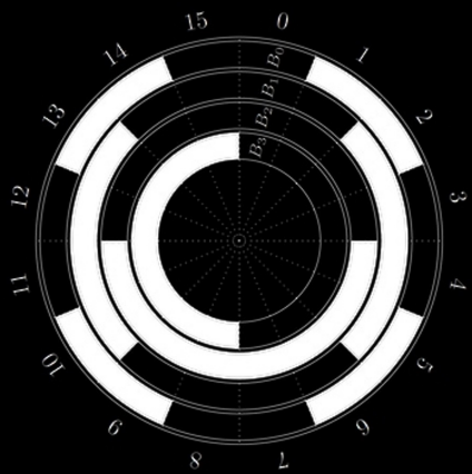
23 Bit Absolute Multi Turn Encoder
