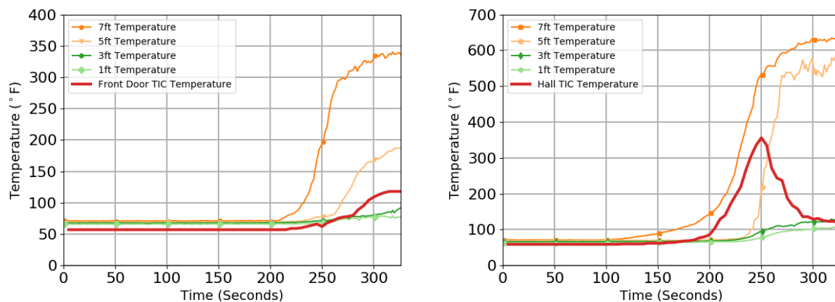
Figure 6.67: Comparison of thermal imager temperature read out to the actual compartment temperatures. Thermal imager from the door location is left and thermal imager from the hallway location is right. The thermocouple temperatures from the adjacent arrays are shown at 7, 5, 3, and 1 ft above the floor (AF). (Experiment 12)
