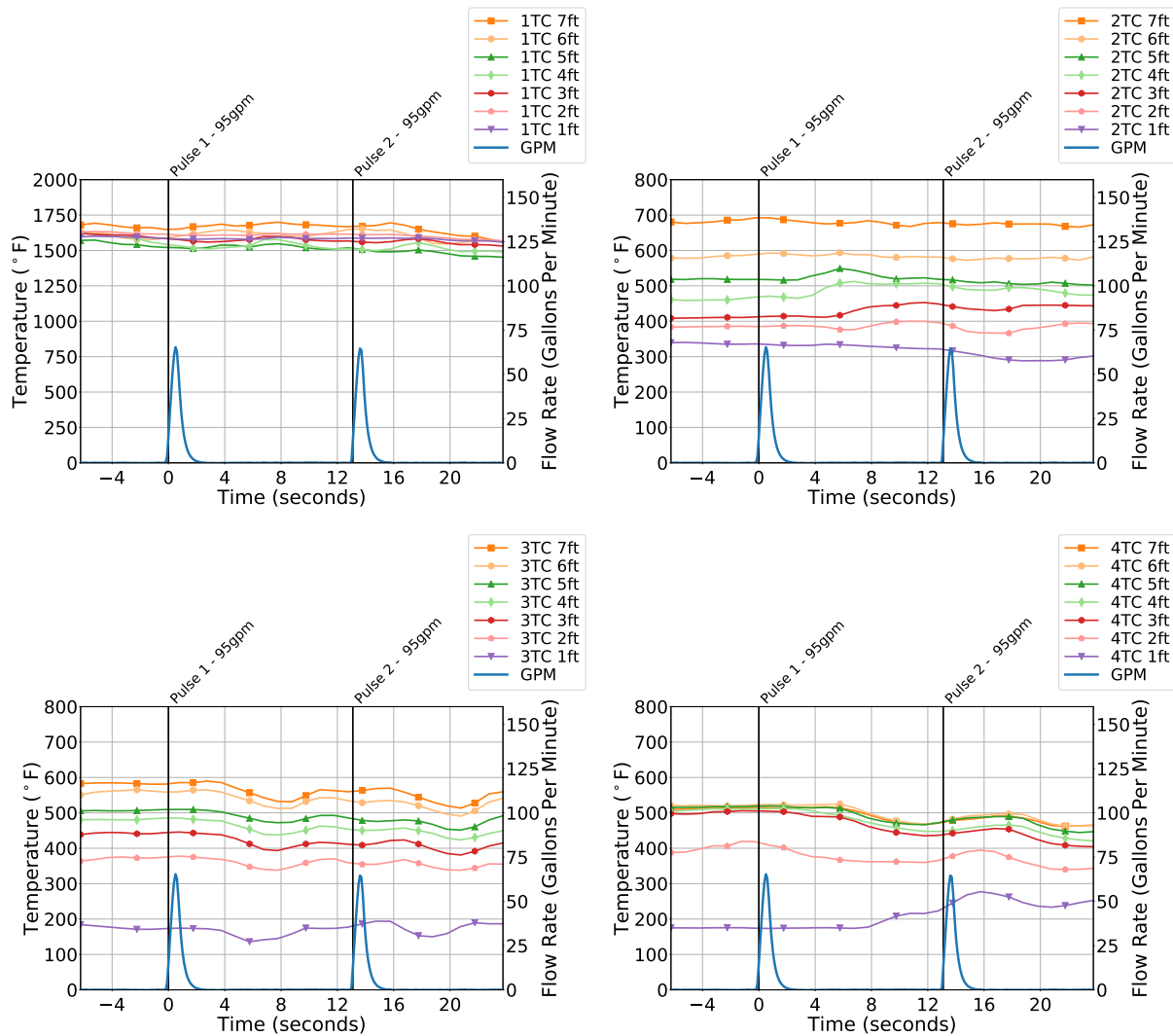
Figure 6.51: Effectiveness of ‘pulse’ technique using 95 gpm nozzle at gas cooling. Upper left is fire compartment, upper left is left center of doorway, lower left is right center of doorway and lower right is just to the right of the advancing hose team.
