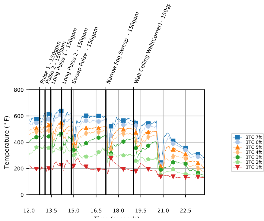
Figure E.935: Experiment 25 - 3 T C 1 2min to End
