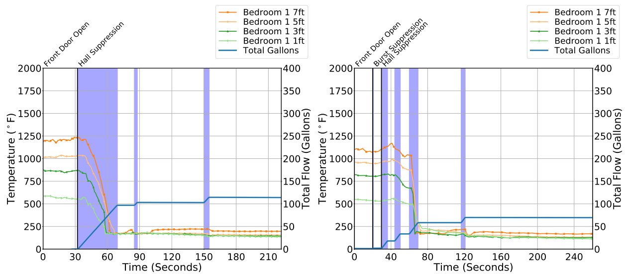
Figure 7.25: Fire room (Bedroom 1) temperatures (1TC) for the two attack methods used in the single room of fire with no ventilation. The blue shaded areas represent water flow from the hose stream. The left shows a “flow and move” method from Experiment 2 and the right shows the “shutdown and move” method from Experiment 6.
