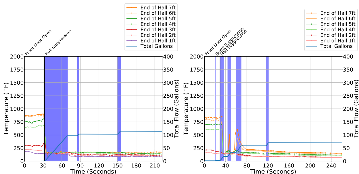
Figure 6.35: End of hallway temperatures (3TC) for the two attack methods used in the single room of fire with no ventilation. The blue shaded areas represent water flow from the hose stream. The left shows a “flow and move” method from Experiment 2 and the right shows the “shutdown and move” method from Experiment 6.
