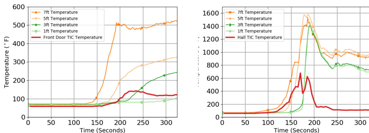
Figure 6.68: Comparison of thermal imager temperature read out to the actual compartment temperatures. Thermal imager from the door location is left and thermal imager from the hallway location is right. The thermocouple temperatures from the adjacent arrays are shown at 7, 5, 3, and 1 ft above the floor (AF). (Experiment 17)
