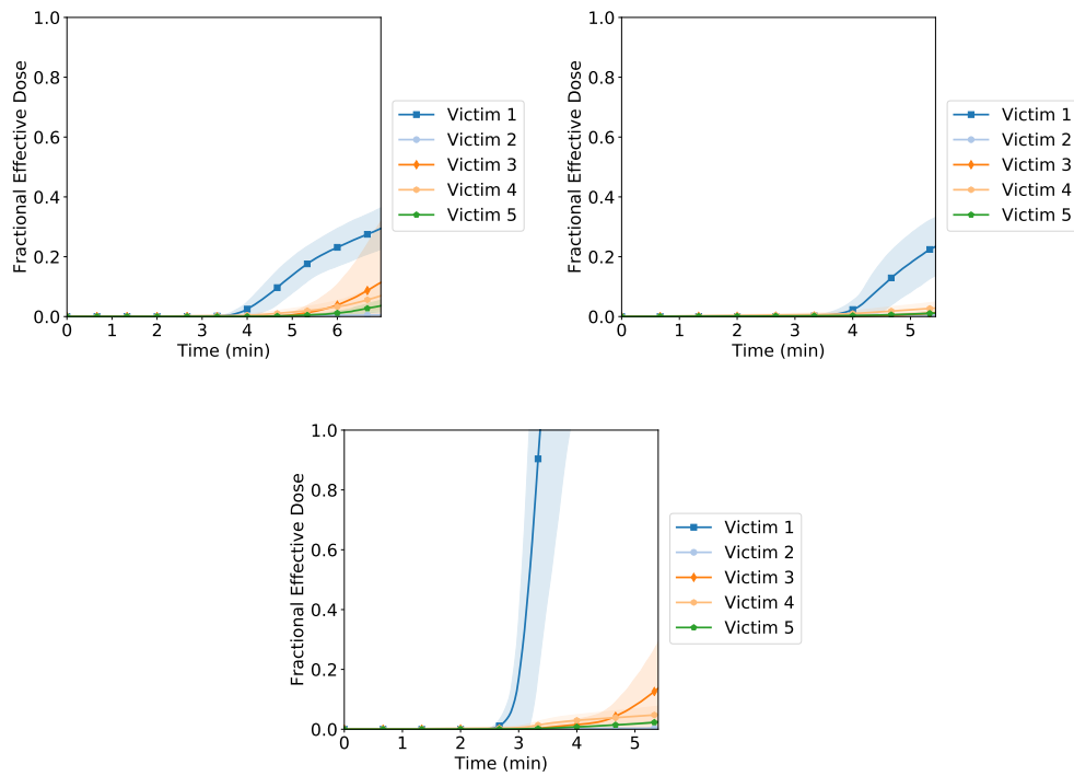
Figure 7.5: Fractional effective dose (FED) of thermal exposure based on total flux to the surface. Top left is the no ventilation case, top right is the single vent with a single room of fire case and bottom is the two rooms of fire with two vent case. The shaded areas represent the various +/- one standard deviation for the average value recorded.
