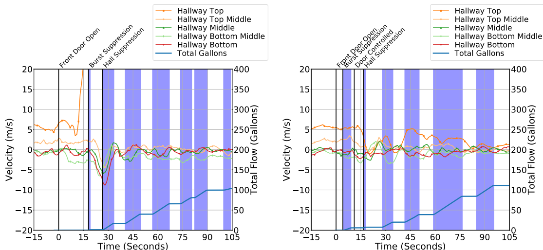
Figure 6.34: Start of hall flow with no door control Experiment 14 (left), with door control Experiment 15 (right) for interior suppression with the window venting prior to initiating the tactic. The blue shaded areas represent where water was flowing from the hose stream. Charts start 15 seconds prior to the tactic is started and continue until 105 seconds after the door was opened.
