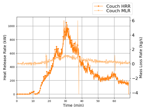
Figure 4.13: Sofa Heat Release Rate Characterization Results
