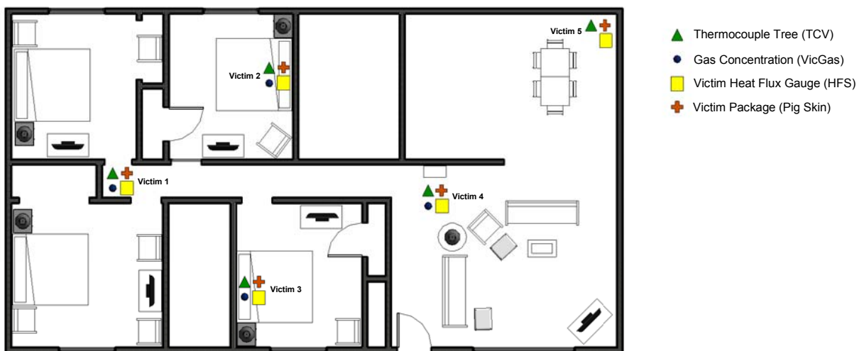
Figure 4.29: Victim Instrumentation Plan
