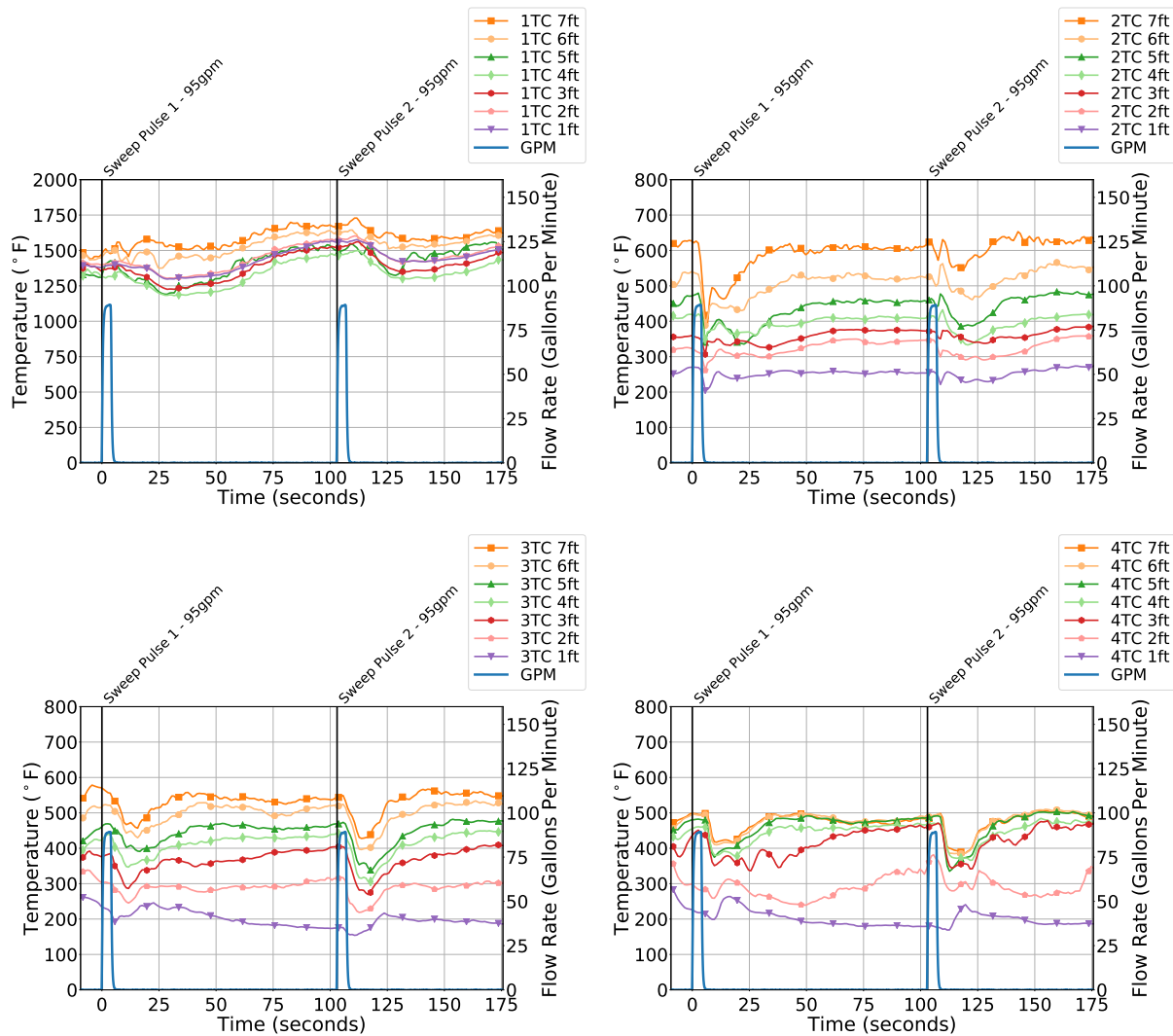
Figure 6.55: Effectiveness of 'sweeping pulse' technique using 95 gpm nozzle at gas cooling. Upper left is fire compartment, upper right is left center of doorway, lower left is right center of doorway and lower right is just to the right of the advancing hose team.
