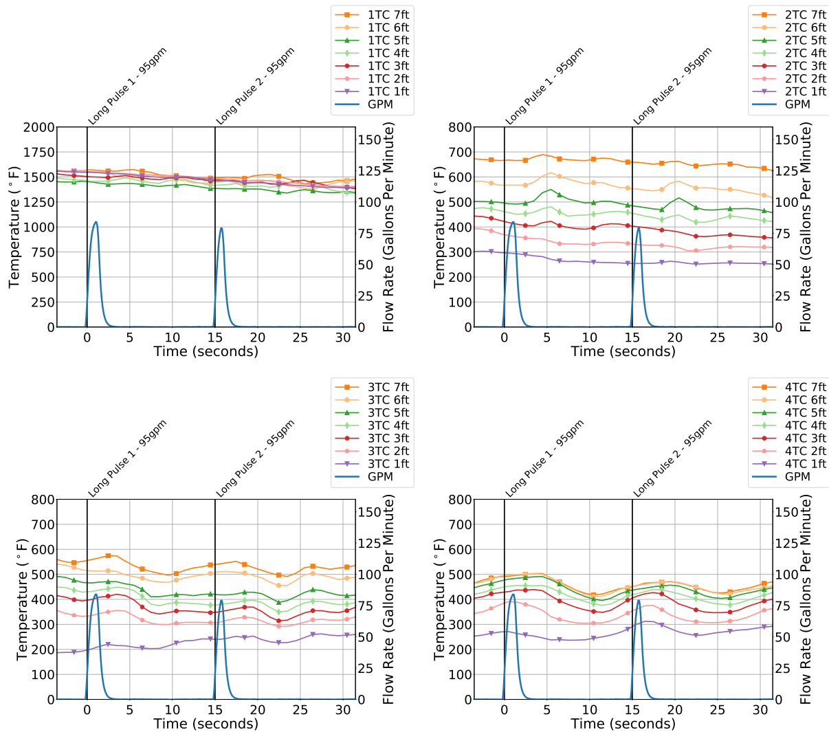
Figure 6.53: Effectiveness of ‘long pulse’ technique using 95 gpm nozzle at gas cooling. Upper left is fire compartment, upper left is left center of doorway, lower left is right center of doorway and lower right is just to the right of the advancing hose team.
