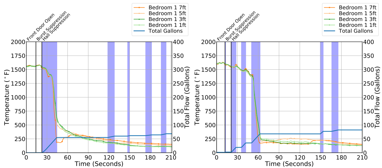
Figure 6.39: Fire room (Bedroom 1) temperatures (1TC) for the two attack methods used in the single room of fire with a window vent opposite the suppression crew. The blue shaded areas represent water flow from the hose stream. The left shows a “flow and move” method from Experiment 9 and the right shows the “shutdown and move” method from Experiment 10.
