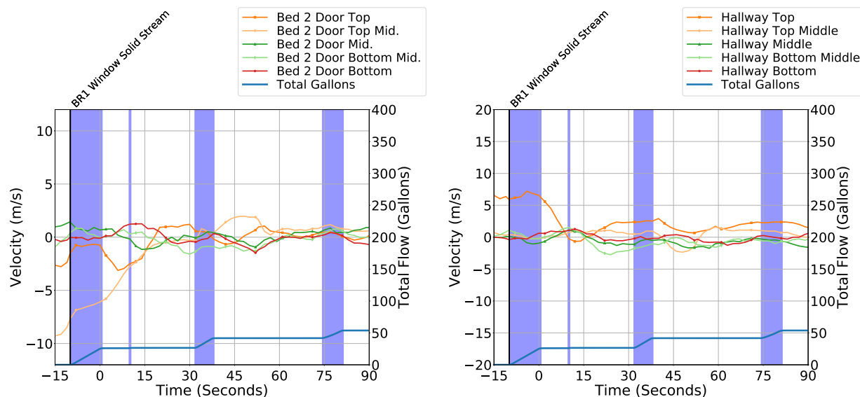
Figure 6.32: Gas velocities at room across from the fire room (left) and the start of hall (right) for exterior water application with straight stream with one room of fire and a single window vent. The front door is closed. The blue shaded areas represent where water was flowing from the hose stream.
