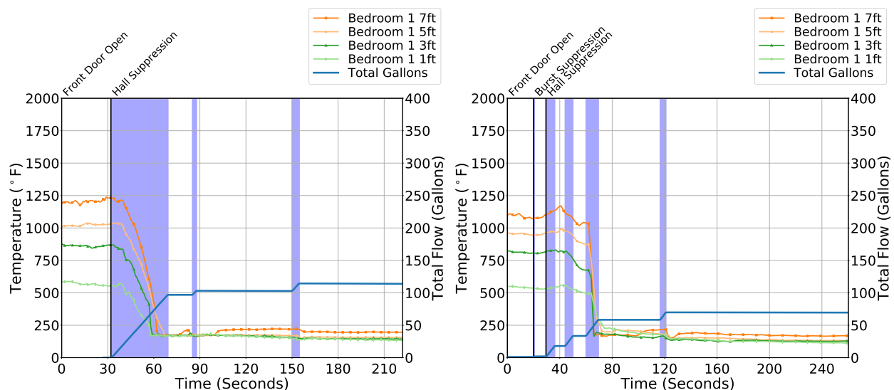
Figure 6.38: Fire room (Bedroom 1) temperatures (1TC) for the two attack methods used in the single room of fire with no ventilation. The blue shaded areas represent water flow from the hose stream. The left shows a “flow and move” method from Experiment 2 and the right shows the “shutdown and move” method from Experiment 6.
