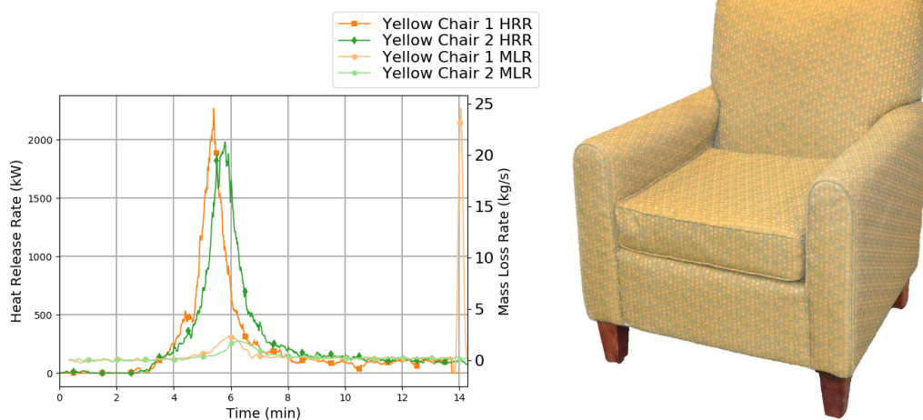
Figure 4.12: Yellow Chair Heat Release Rate Characterization Results
