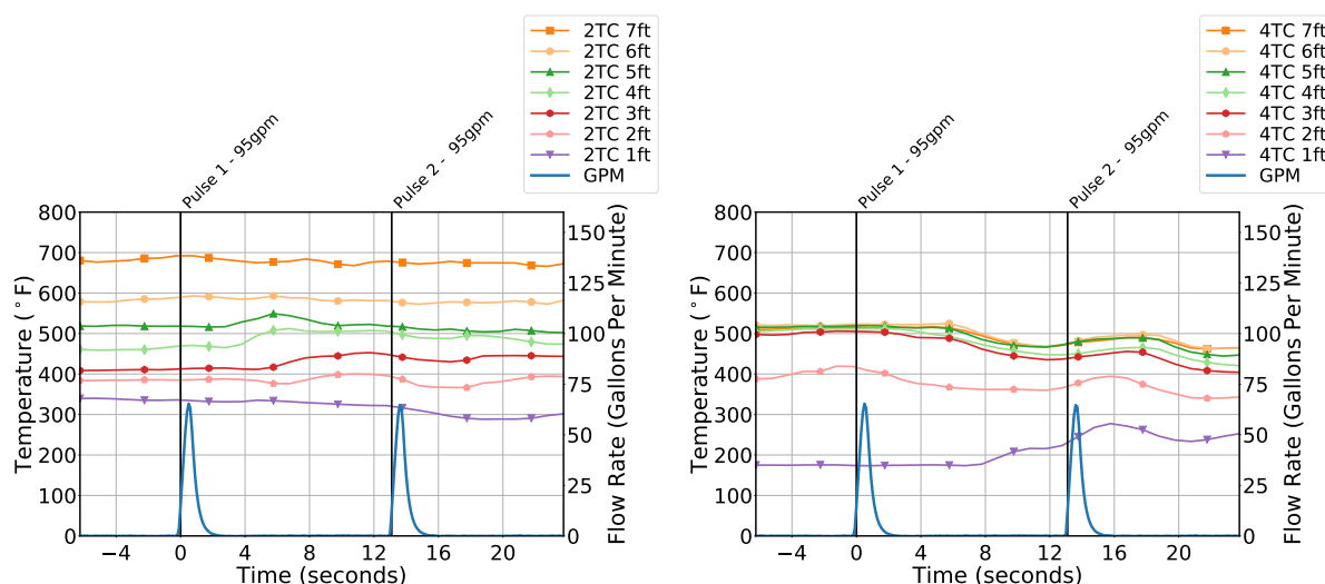
Figure 7.31: Effectiveness of ‘pulse’ technique at gas cooling using 95 gpm nozzle. Left center of doorway (left), right center of doorway (right). (Experiment 25)
