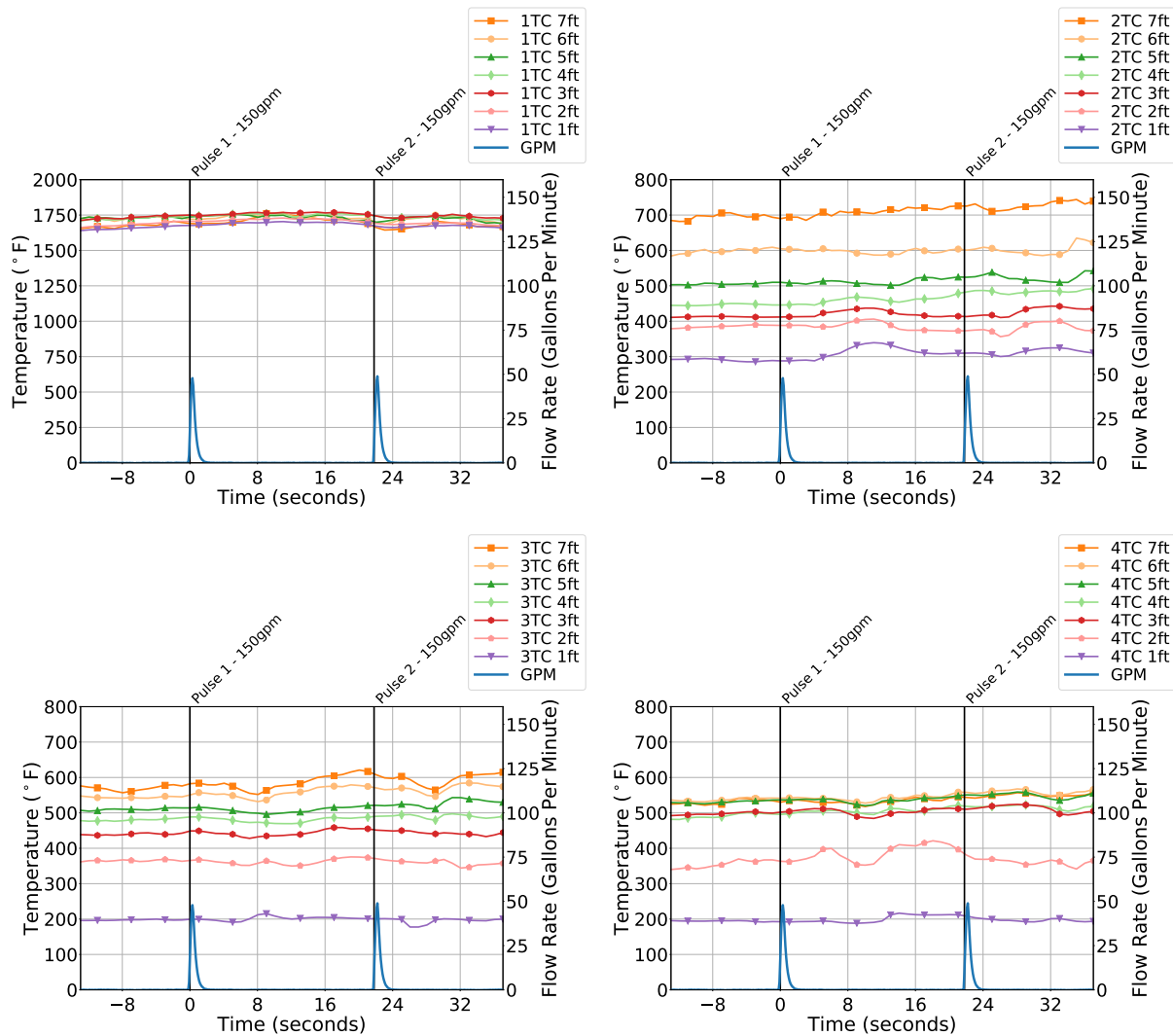
Figure 6.52: Effectiveness of 'pulse' technique using 150 gpm nozzle at gas cooling. Upper left is fire compartment, upper left is left center of doorway, lower left is right center of doorway and lower right is just to the right of the advancing hose team.
