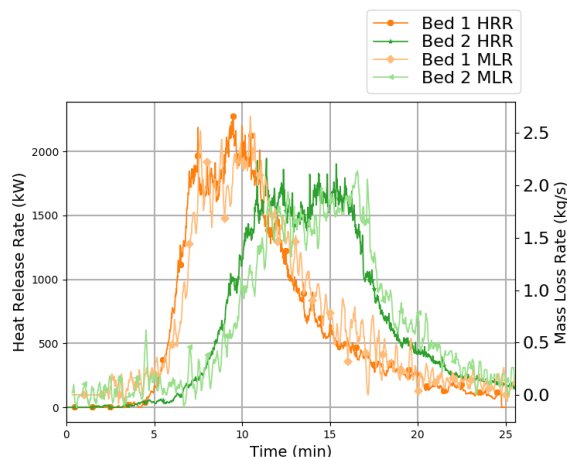
Figure 4.14: Bed Heat Release Rate Characterization Results
