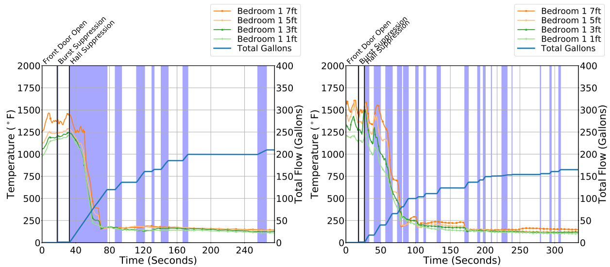
Figure 6.40: Fire room (Bedroom 1) temperatures (1TC) for the two attack methods used in the single room of fire with a window vent opposite the suppression crew. The blue shaded areas represent water flow from the hose stream. The left shows a “flow and move” method from Experiment 13 and the right shows the “shutdown and move” method from Experiment 14.
