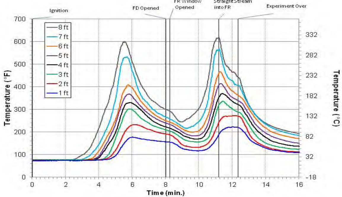
Figure E.1: Experiment 1 Living Room Temperature
