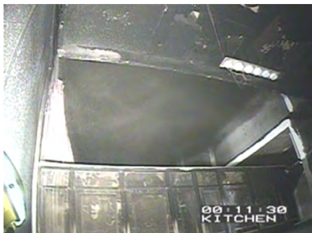
Figure 5.475: Exp. 10 just before roof ventilation looking up to Bedroom fire
