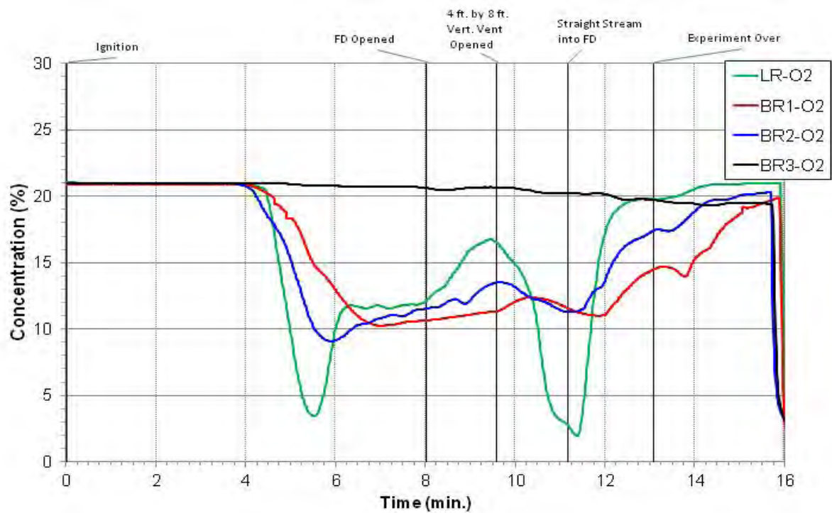
Figure 5.119: Experiment 7 - Oxygen Concentration
