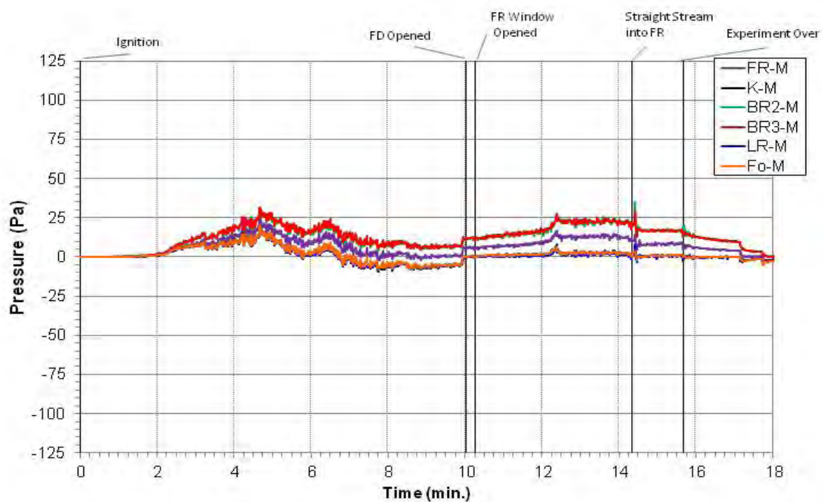
Figure 5.237: Experiment 2 - Middle Pressure
