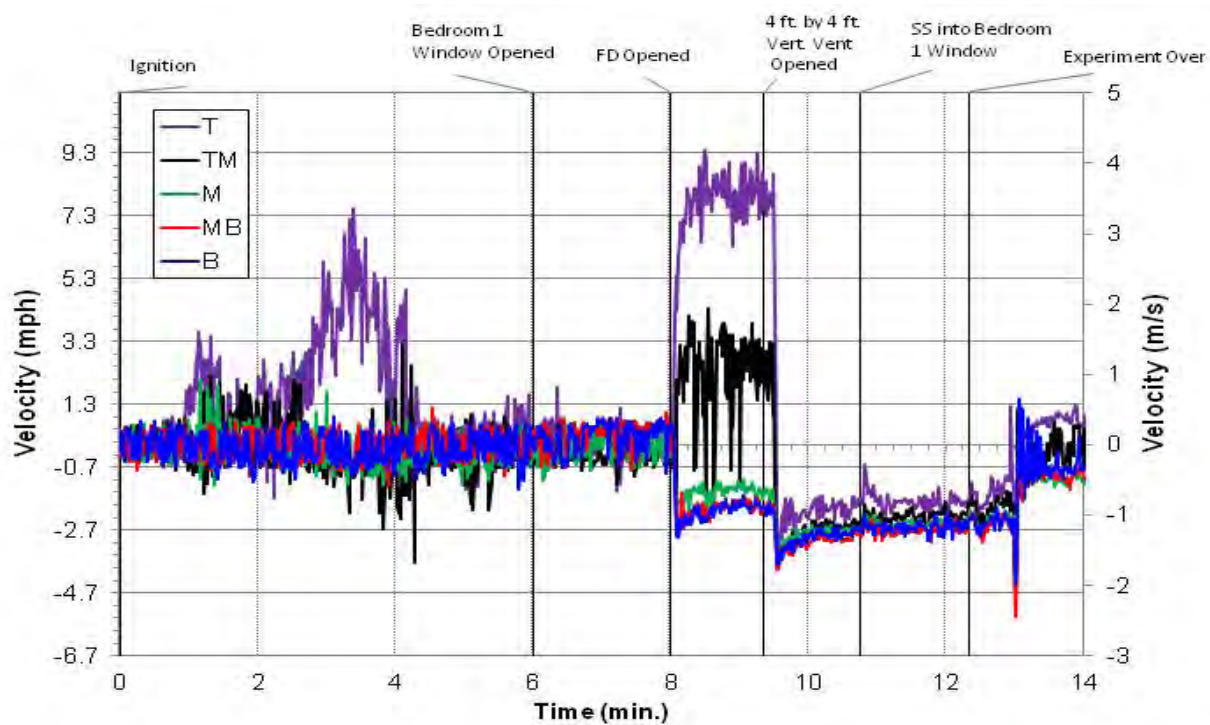
Figure 5.162: Experiment 11 - Front Door Velocity
