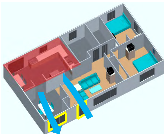
Figure 5.529: Flow Path with Water Flow through Front Door with Dining Room Window Open
