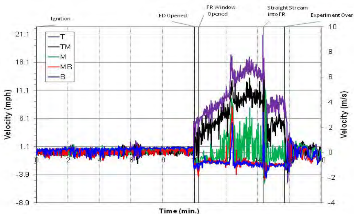
Figure 5.242: Experiment 2 - Front Door Velocity
