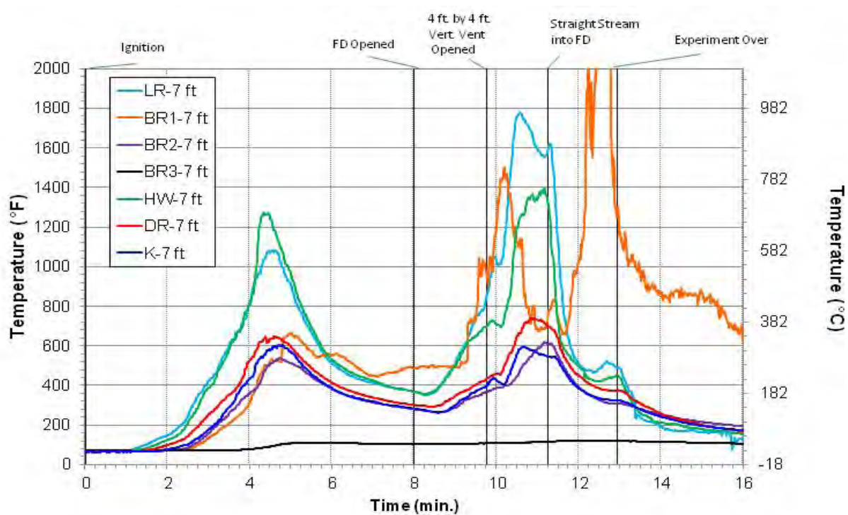
Figure 5.92: Experiment 5 - 7 ft. Temperatures
