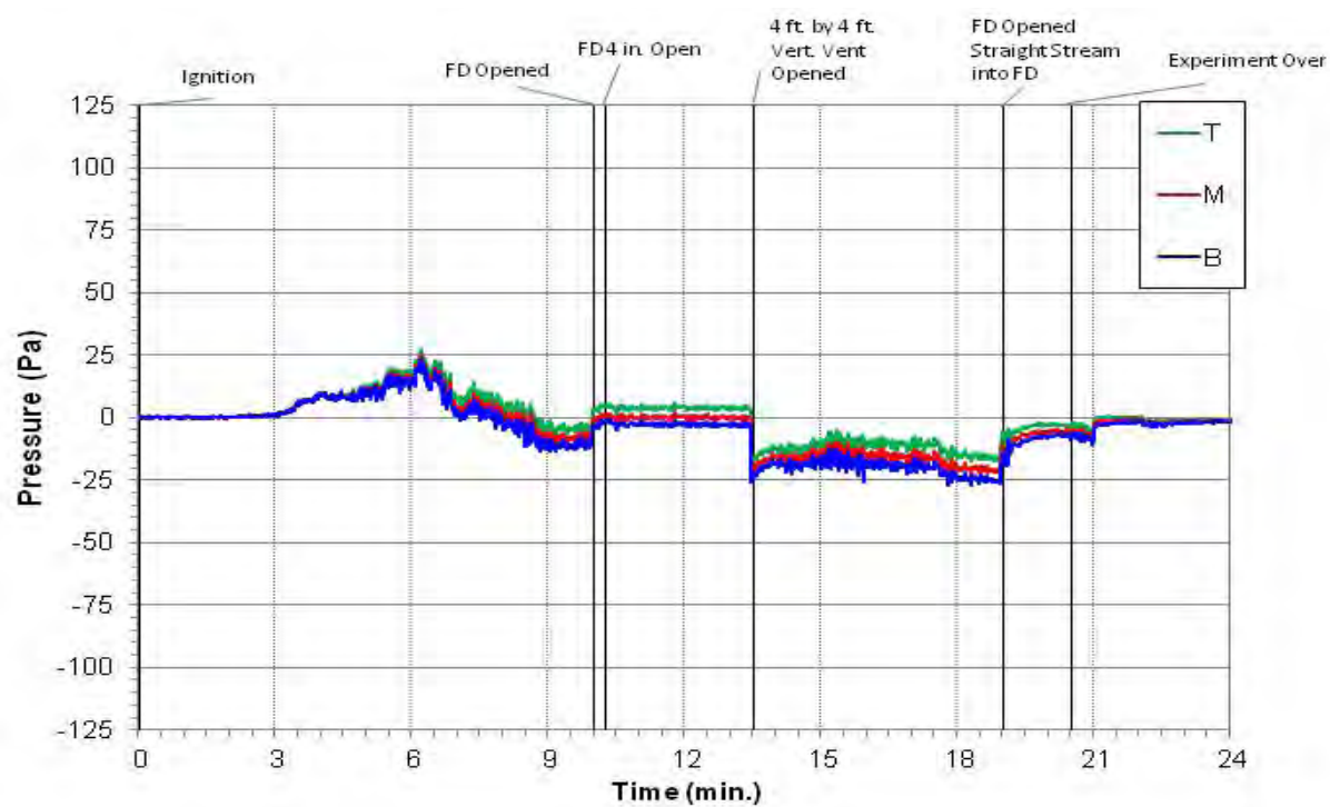
Figure E.81: Experiment 4 Kitchen Pressure
