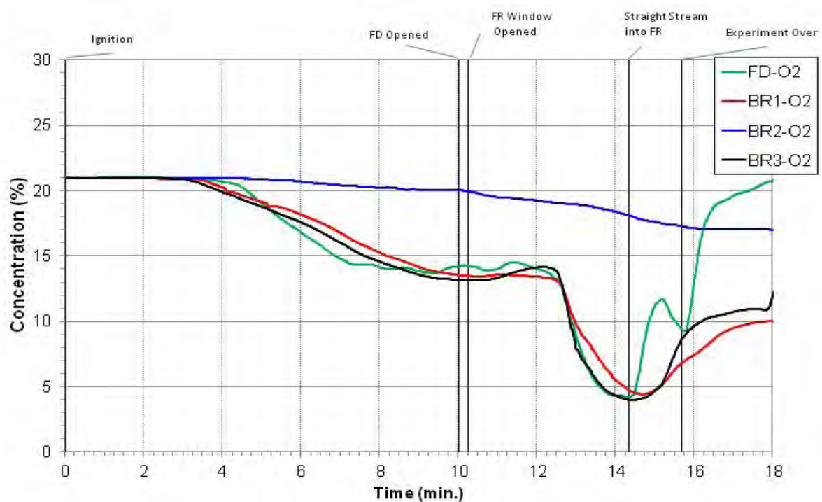
Figure 5.239: Experiment 2 - Oxygen Concentration
