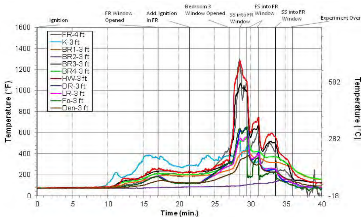
Figure 5.381: Experiment 16 - 3 ft. Temperatures
