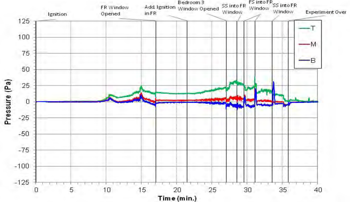
Figure E.345: Experiment 16 Family Room Pressure
