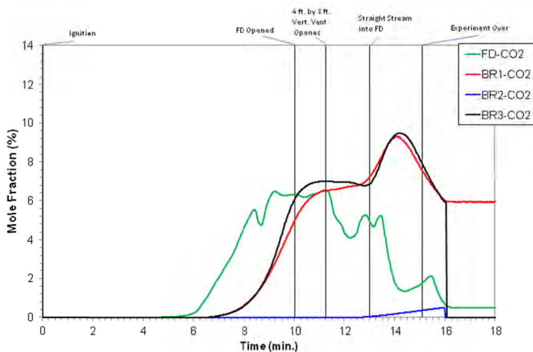
Figure 5.490: CO 2 Measurements in Two-Story Structure from Experiment 8
