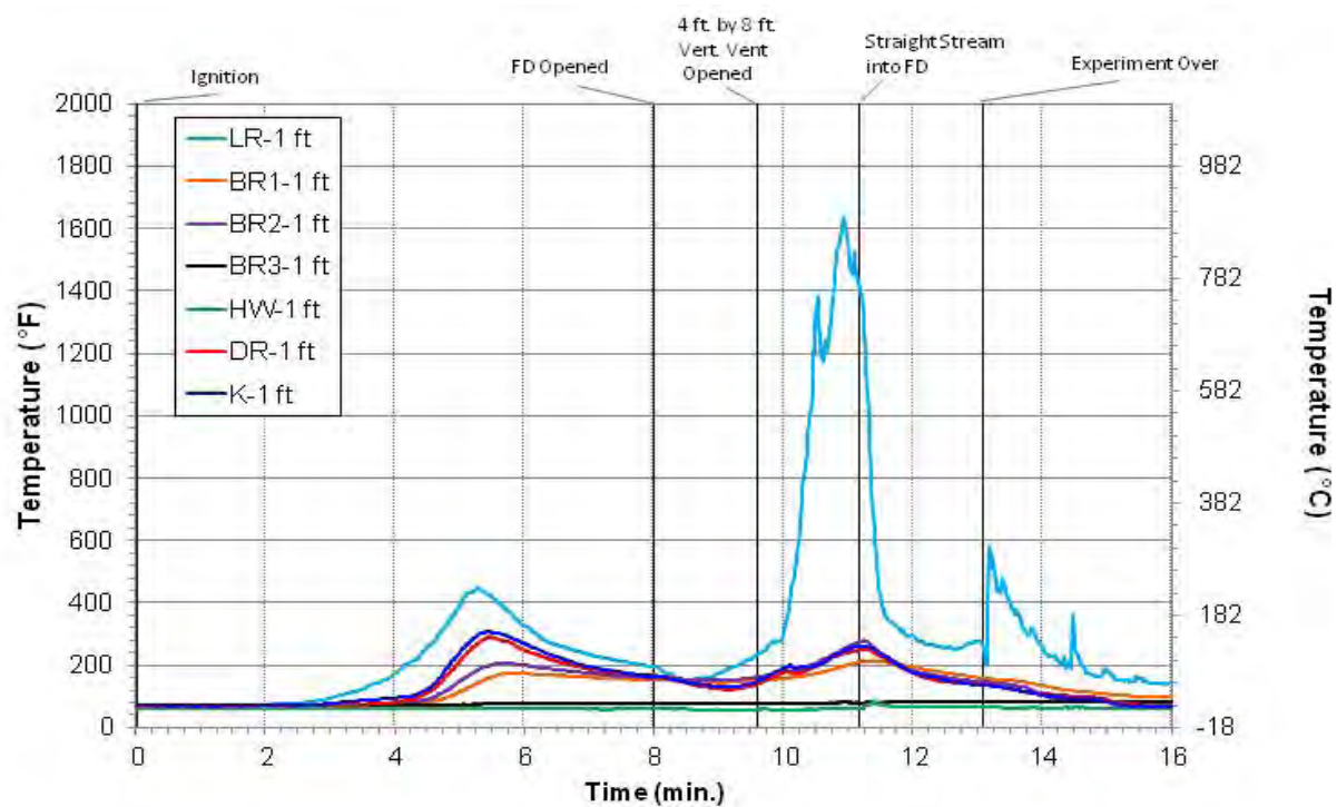
Figure 5.115: Experiment 7 - 1 ft. Temperatures
