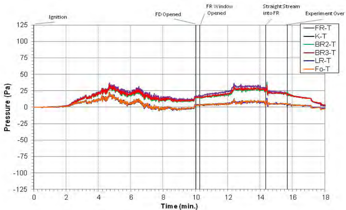
Figure 5.238: Experiment 2 - Top Pressure
