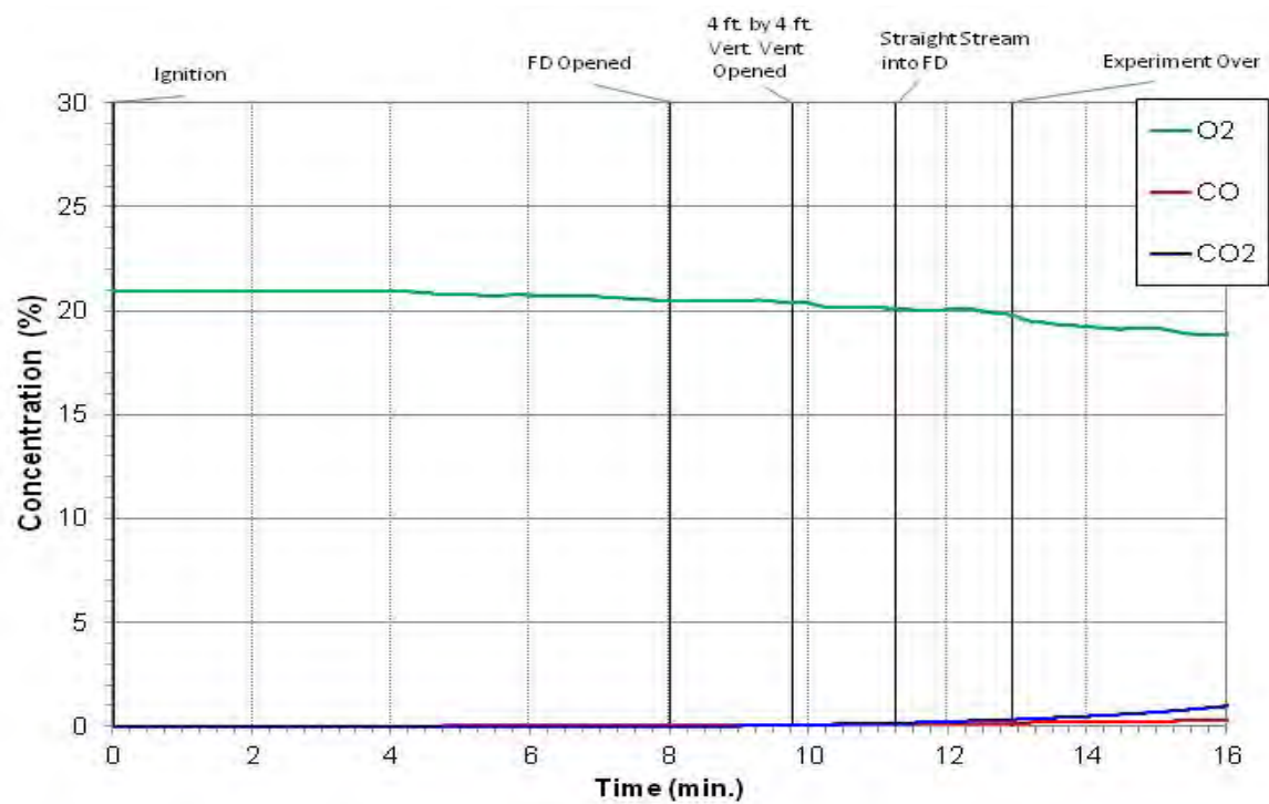
Figure E.109: Experiment 5 Bedroom 3 Gas
