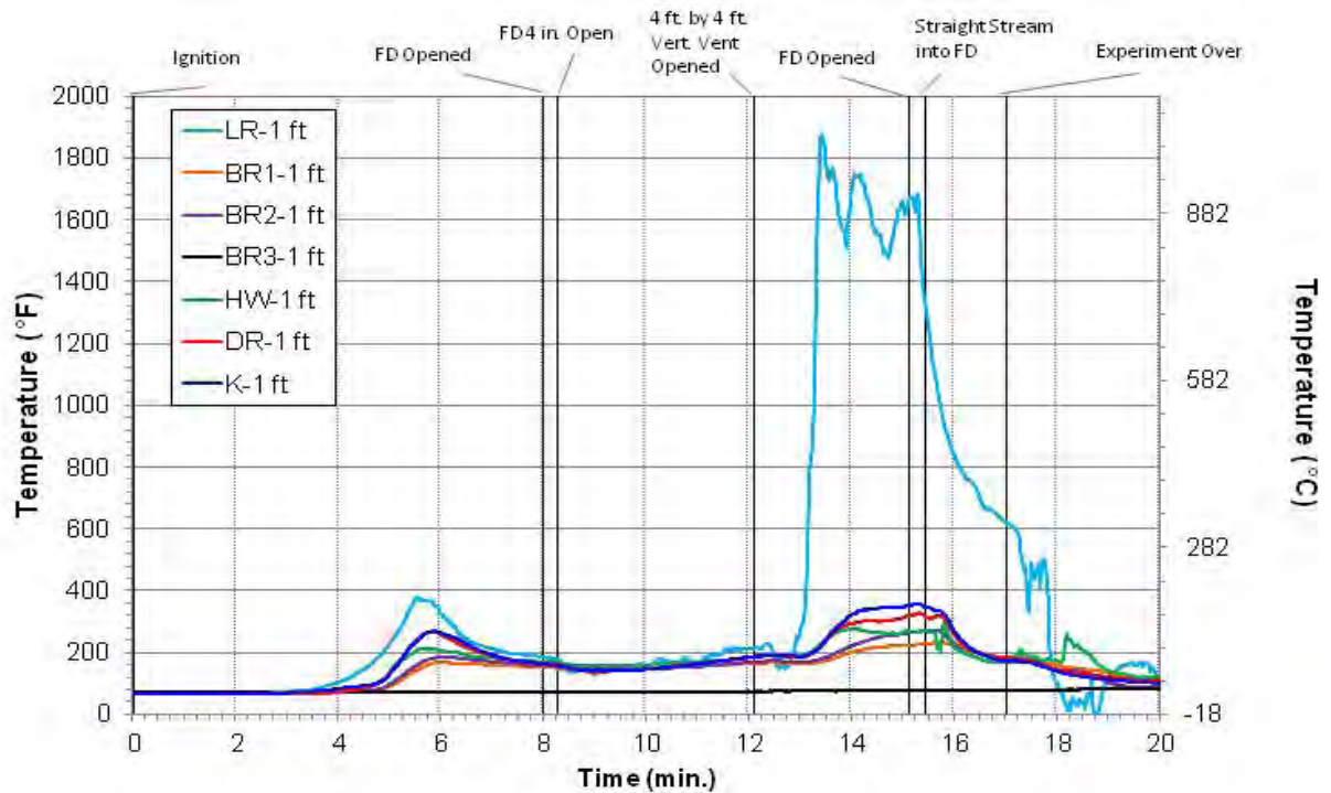
Figure 5.75: Experiment 3 - 1 ft. Temperatures
