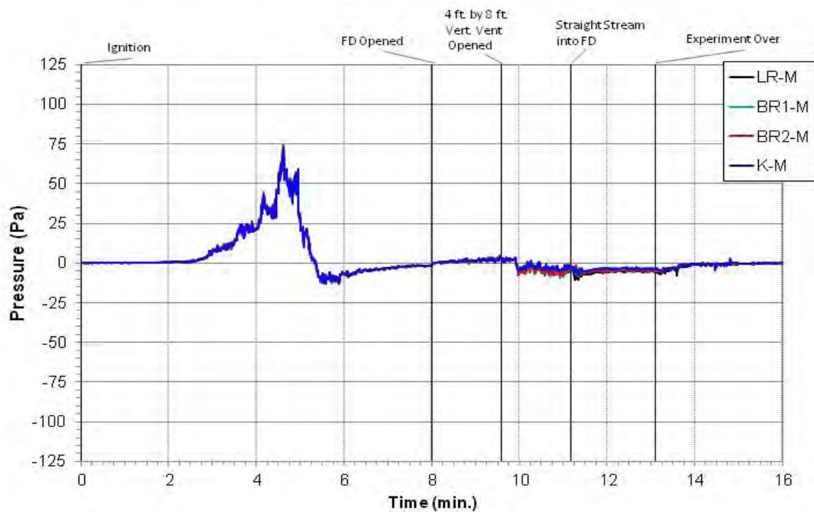
Figure 5.117: Experiment 7 - Middle Pressure
