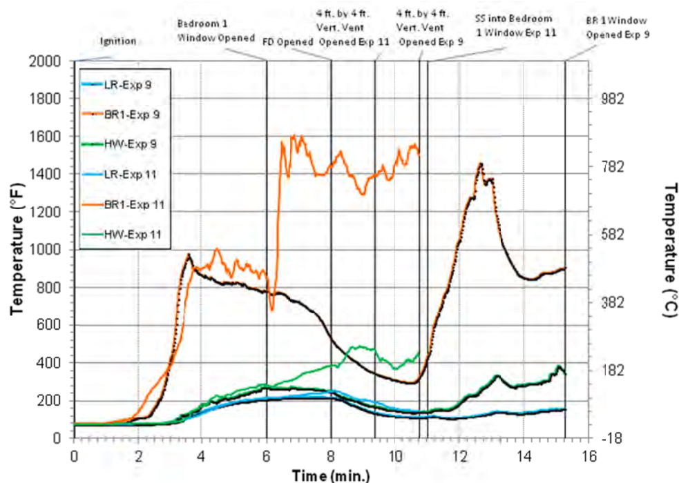
Figure 5.466: Comparison of 3 ft. Temperatures
