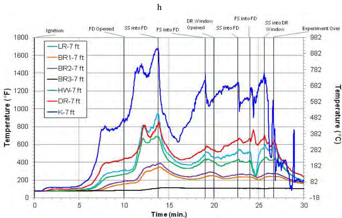
Figure 5.175: Experiment 13 - 7 ft. Temperatures
