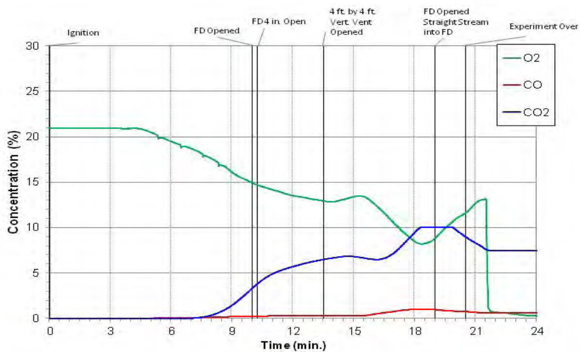
Figure E.87: Experiment 4 Bedroom 1 Gas
