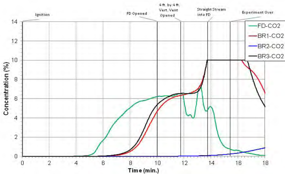
Figure 5.281: Experiment 6 - Carbon Dioxide Concentration
