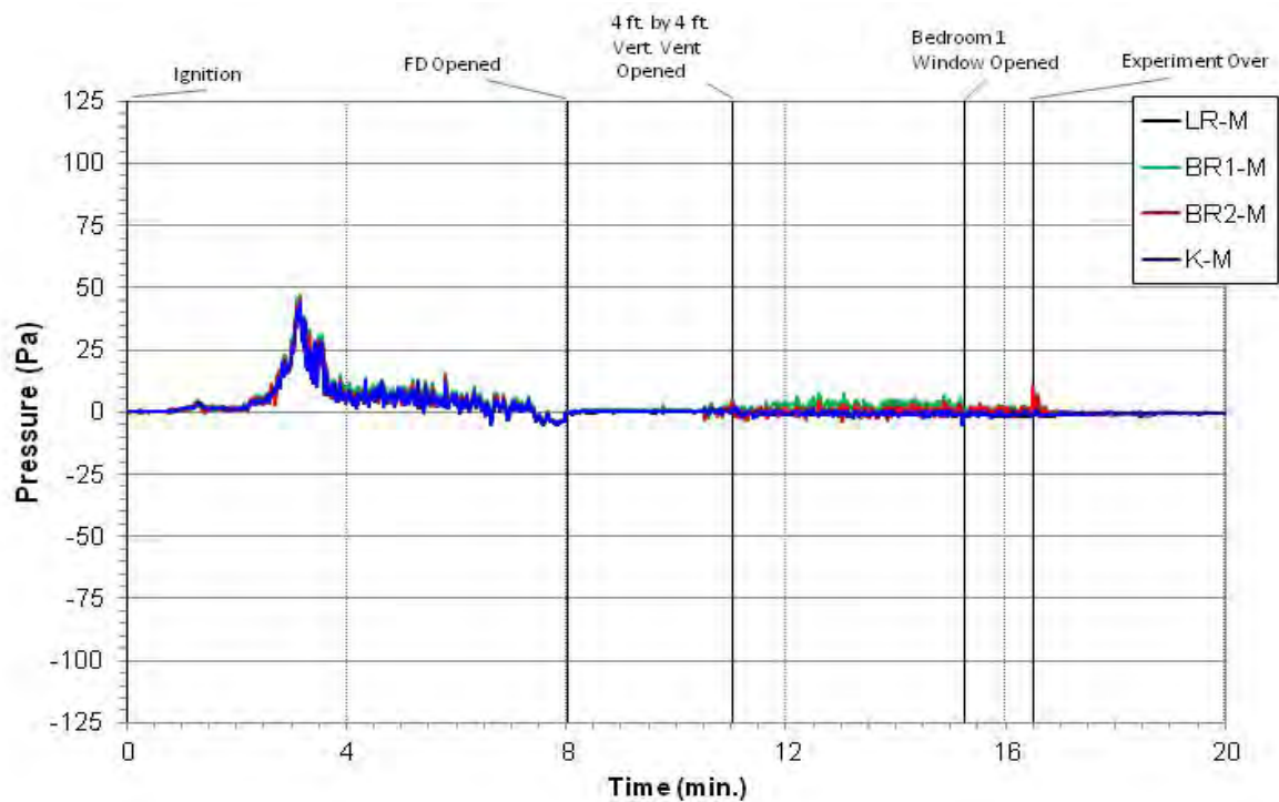
Figure 5.136: Experiment 9 - Middle Pressure
