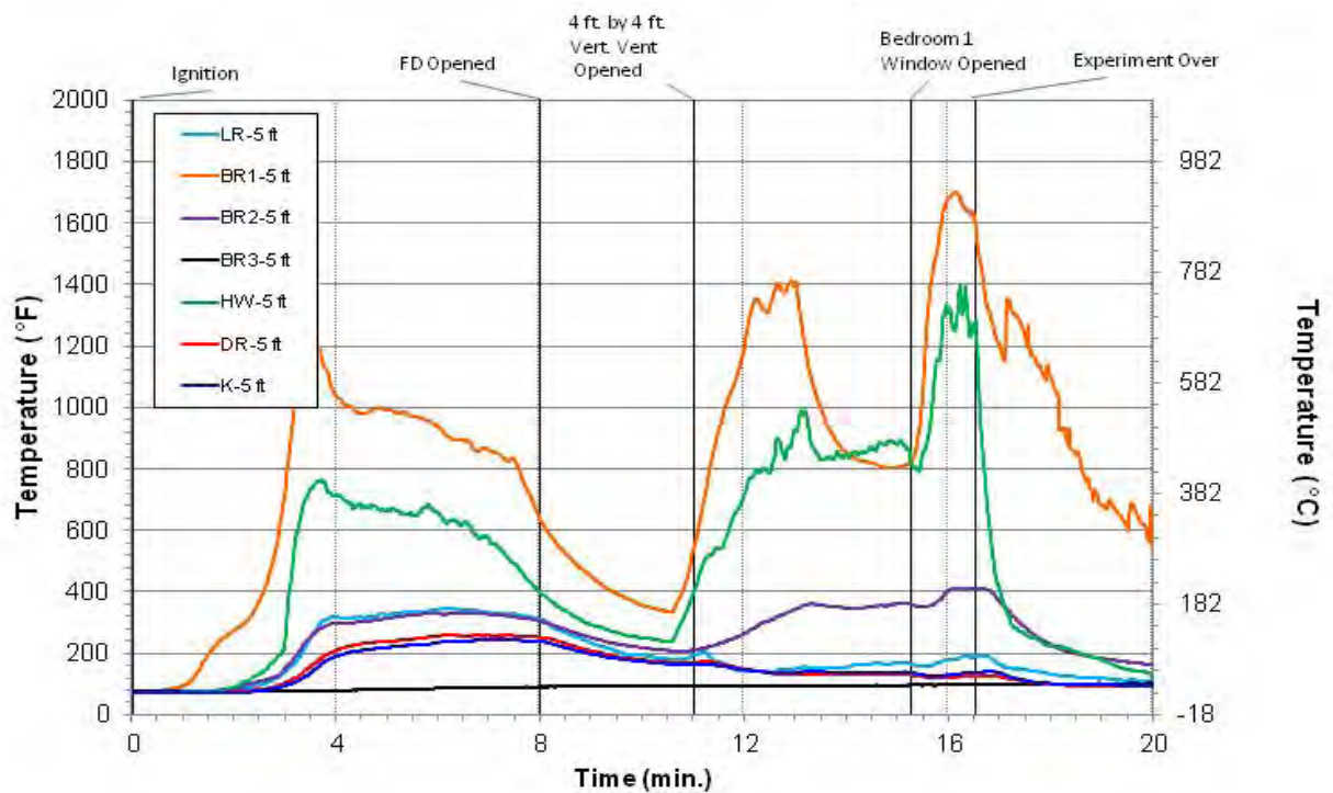
Figure 5.132: Experiment 9 - 5 ft. Temperatures
