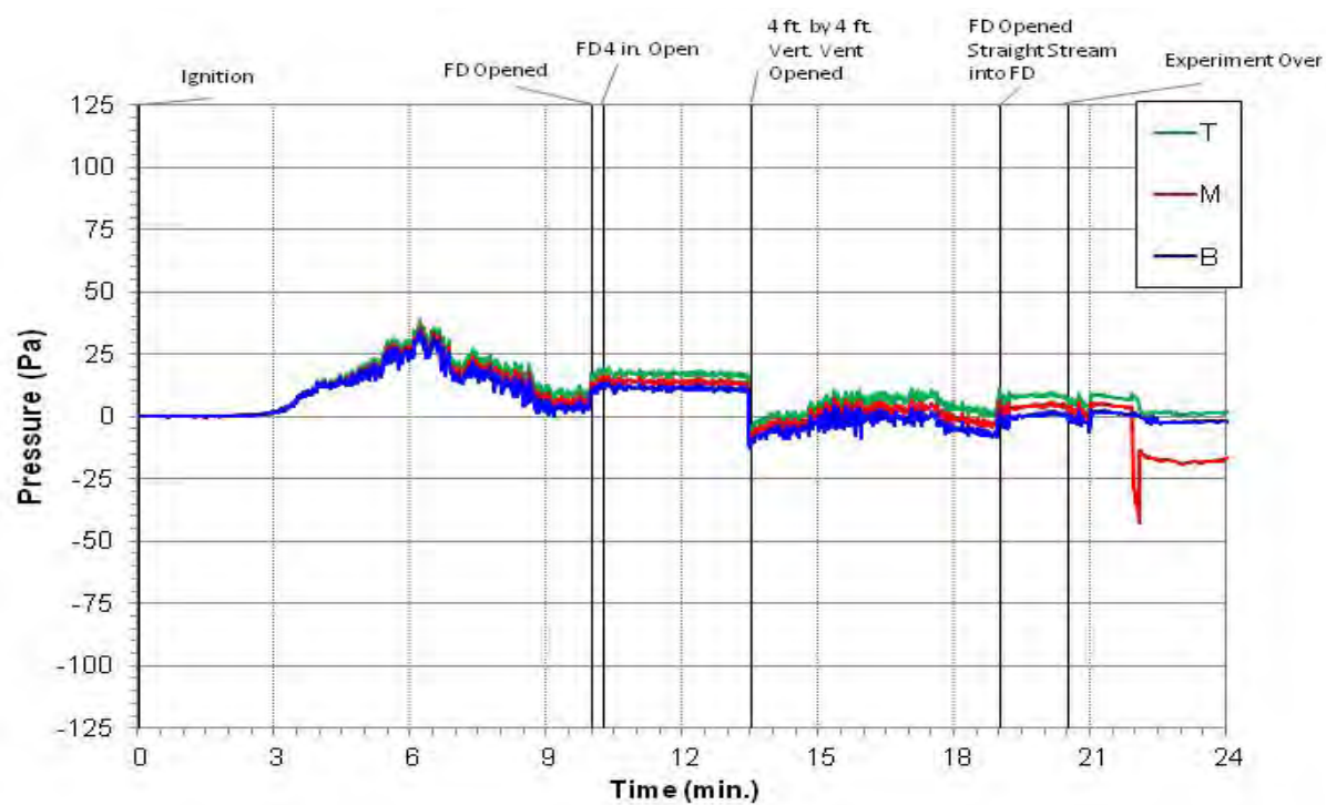
Figure E.79: Experiment 4 Bedroom 2 Pressure
