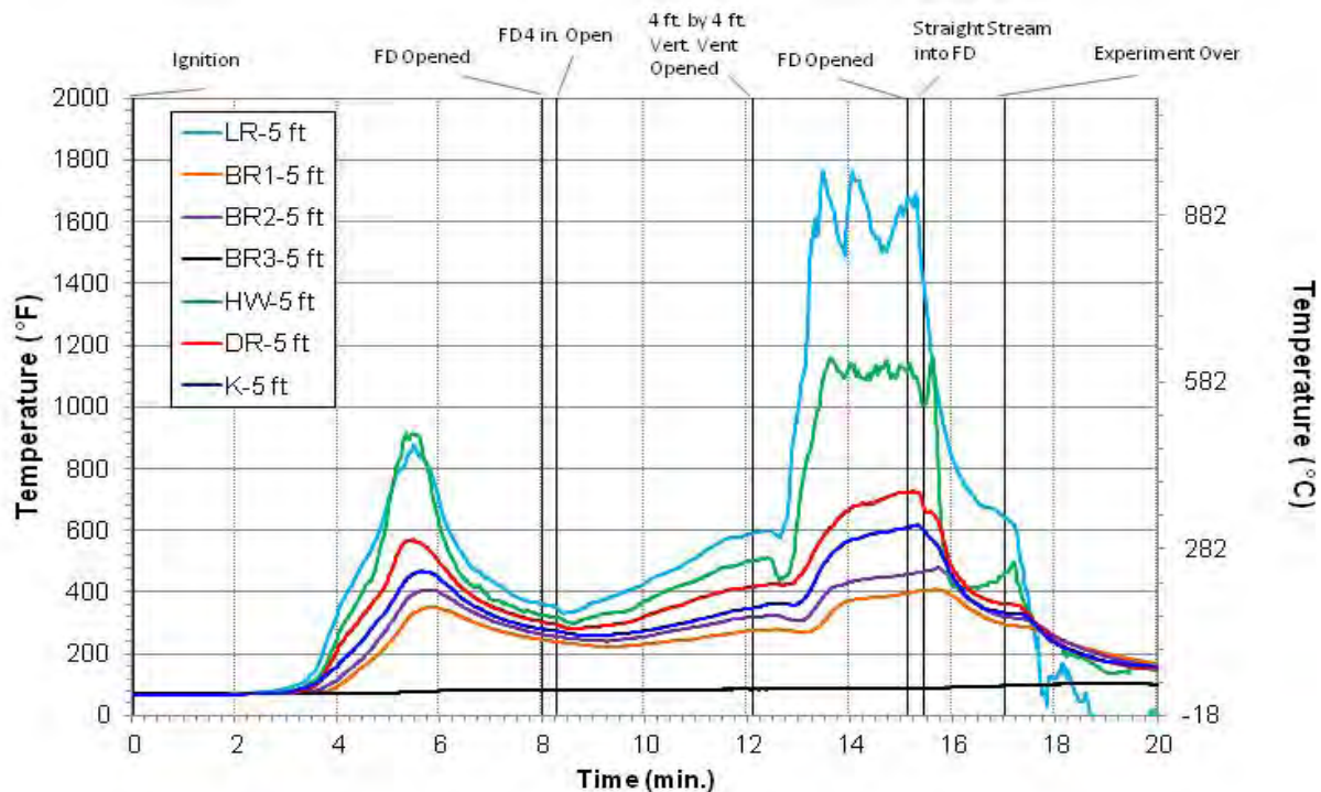
Figure 5.73: Experiment 3 - 5 ft. Temperatures
