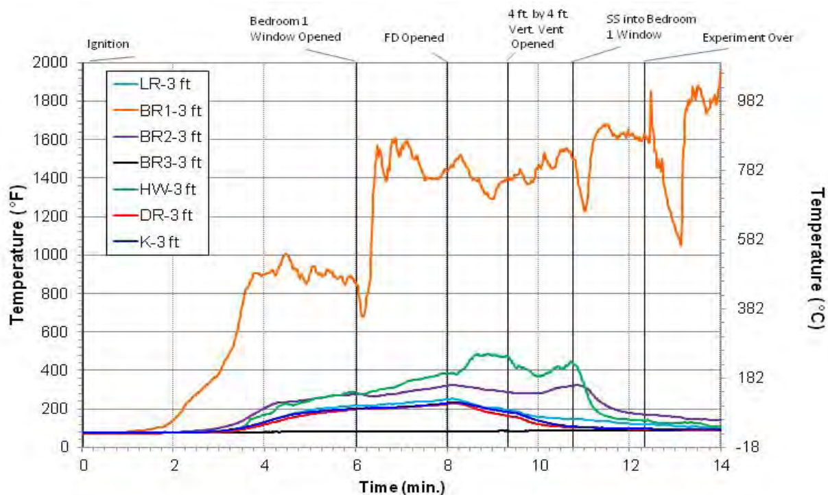
Figure 5.154: Experiment 11 - 3 ft. Temperatures
