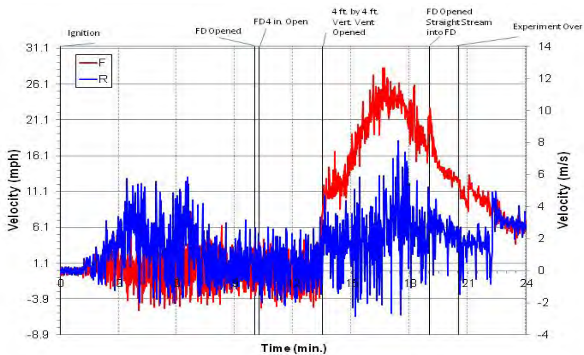
Figure E.85: Experiment 4 Vent Velocity
