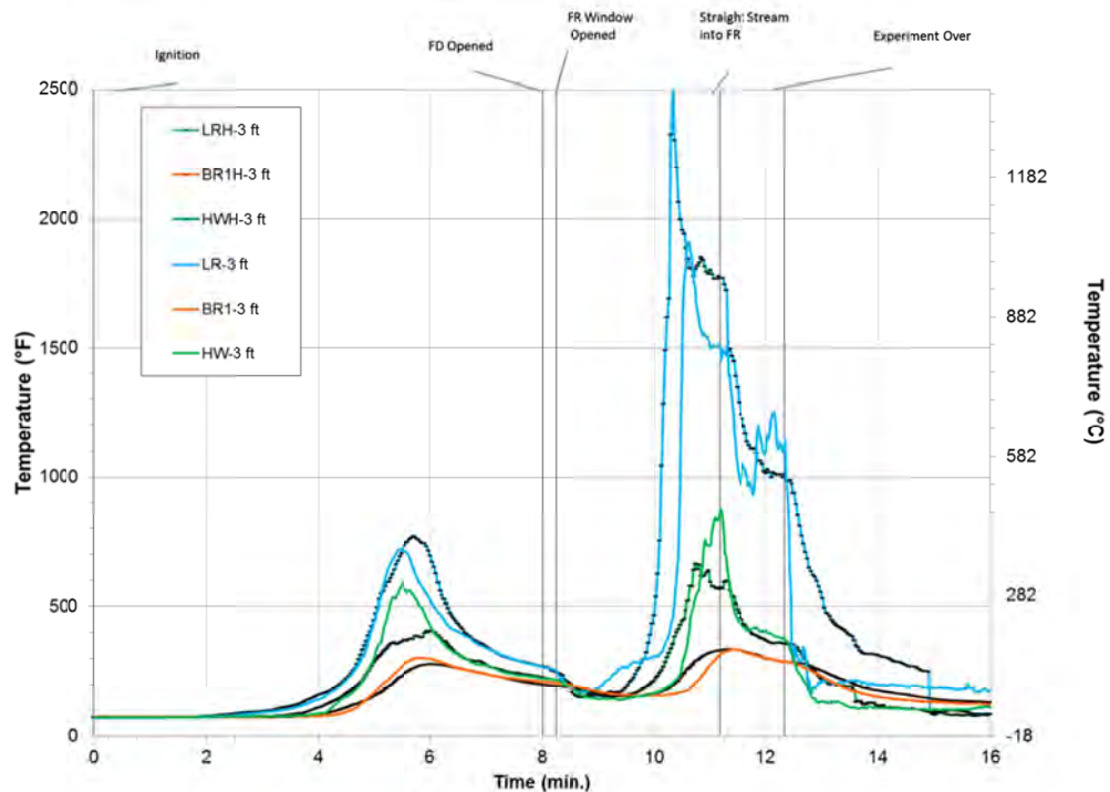
Figure 5.394: Comparison of 3 ft. Temperatures
