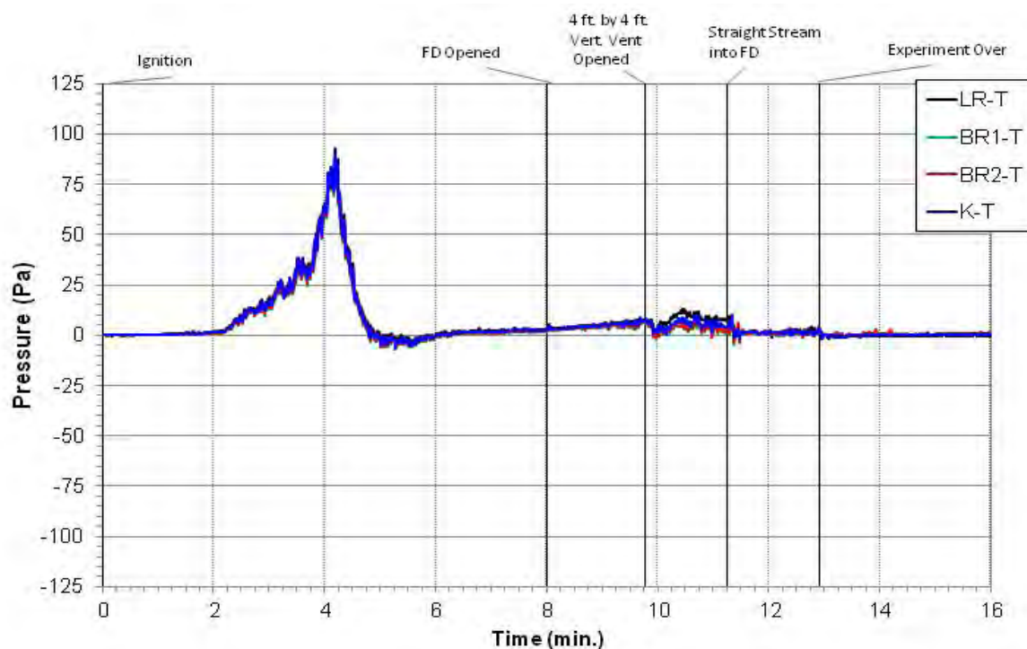
Figure 5.97: Experiment 5 - Middle Pressure
