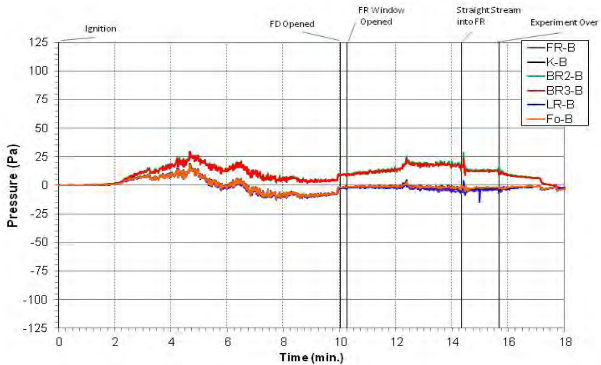
Figure 5.236: Experiment 2 - Bottom Pressure
