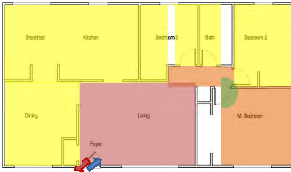
Figure 6.17: Flow path after the living room reaches flashover
