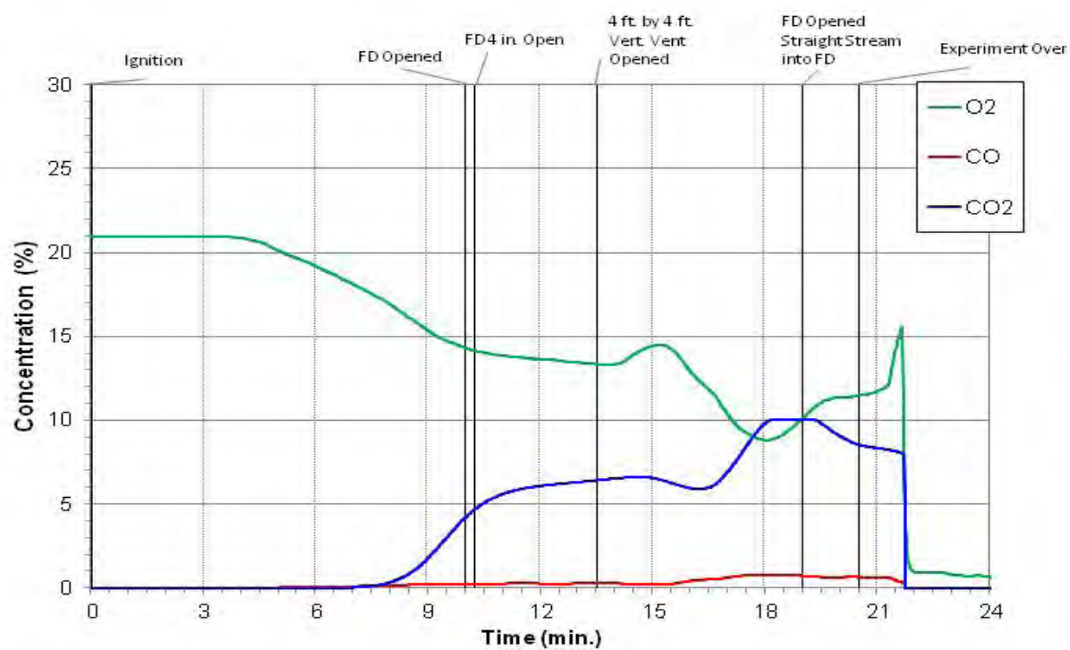
Figure E.89: Experiment 4 Bedroom 3 Gas
