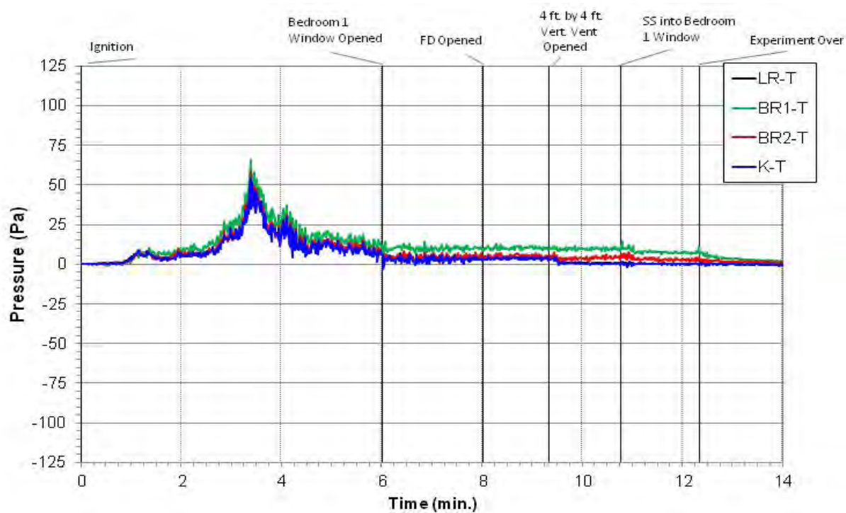
Figure 5.158: Experiment 11 - Top Pressure
