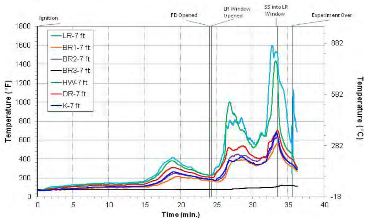
Figure 5.213: Experiment 17 - 7 ft. Temperatures
