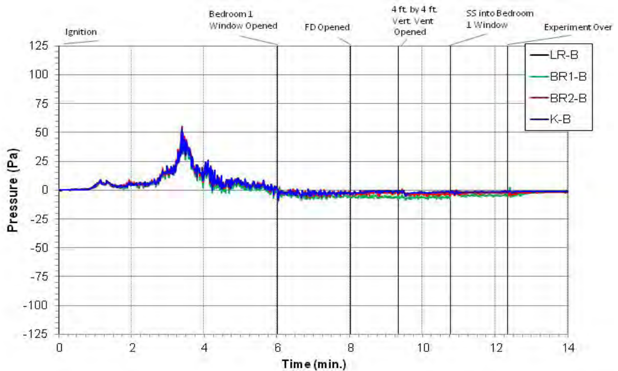
Figure 5.156: Experiment 11 - Bottom Pressure
