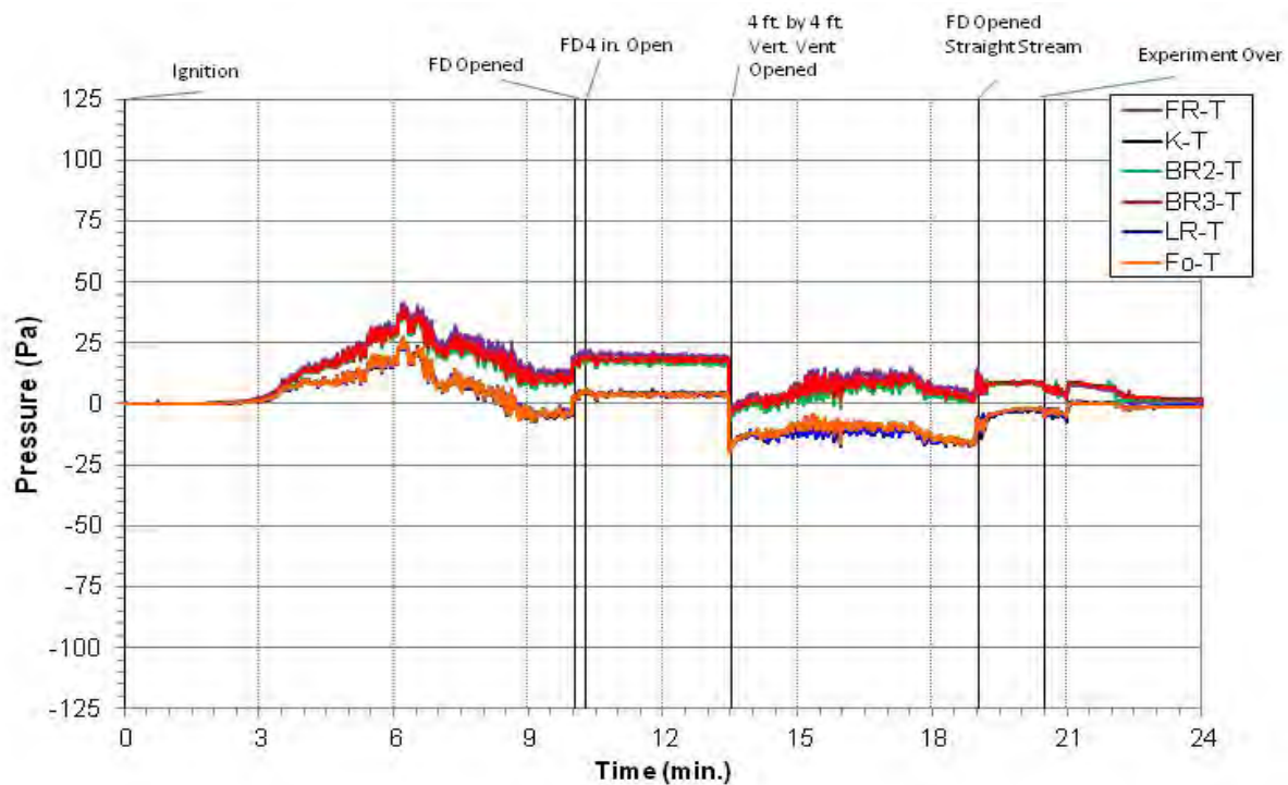
Figure 5.258: Experiment 4 - Top Pressure
