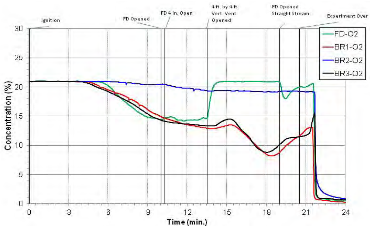
Figure 5.259: Experiment 4 - Oxygen Concentration
