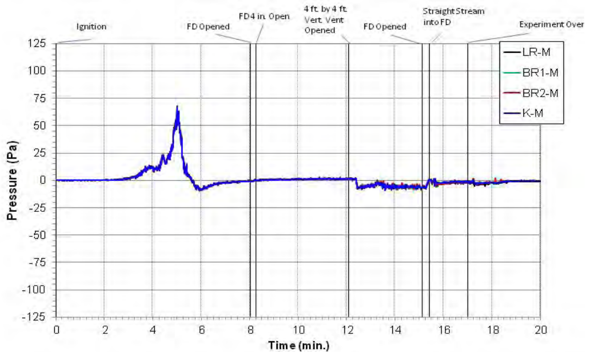
Figure 5.77: Experiment 3 - Middle Pressure
