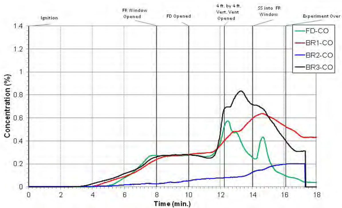
Figure 5.341: Experiment 12 - Carbon Monoxide Concentration
