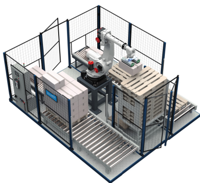
ALPHA PALLETIZER
